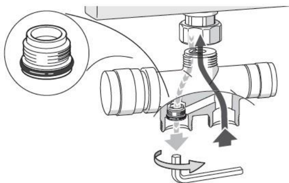
BITUBO (TWO PIPE SYSTEM)
